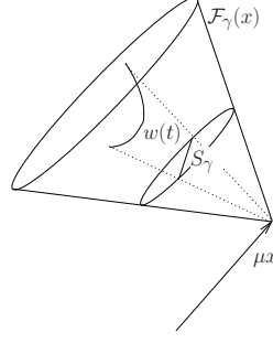
FIG. 4.2. The line segment S_\gamma(x) and the curve w(t) .
