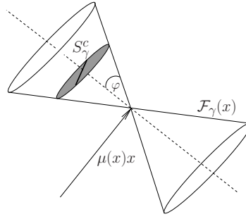
FIG. 2.2. The cross section S_\gamma^c and the line segment S_\gamma (bold line).
